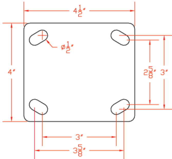
Top Mounting Plate
